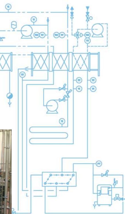
Pasteurising System
